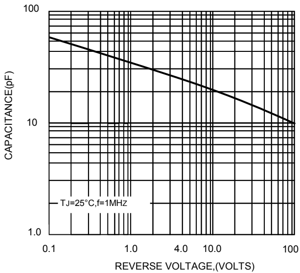
FIG.3-TYPICAL JUNCTION CAPACITANCE
